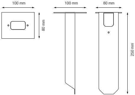
Spike
